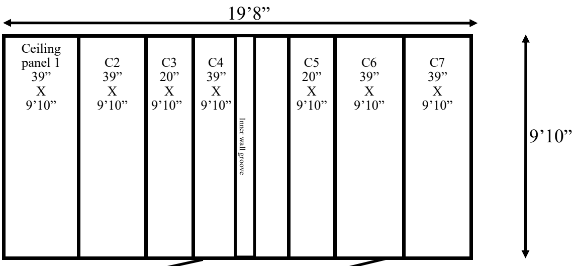
9'10" x 19'8" x 8' H Ready Ship Combo Cooler / Freezer Wall, Ceiling & Floor Panels Diagrams
